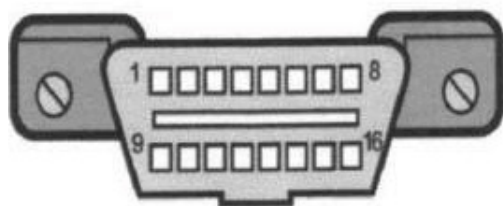
Female Connector (Plug at the car)
