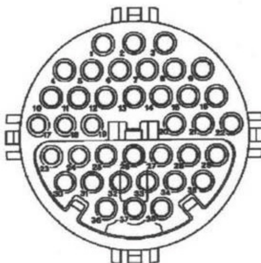
Female Connector (Plug at the car)
