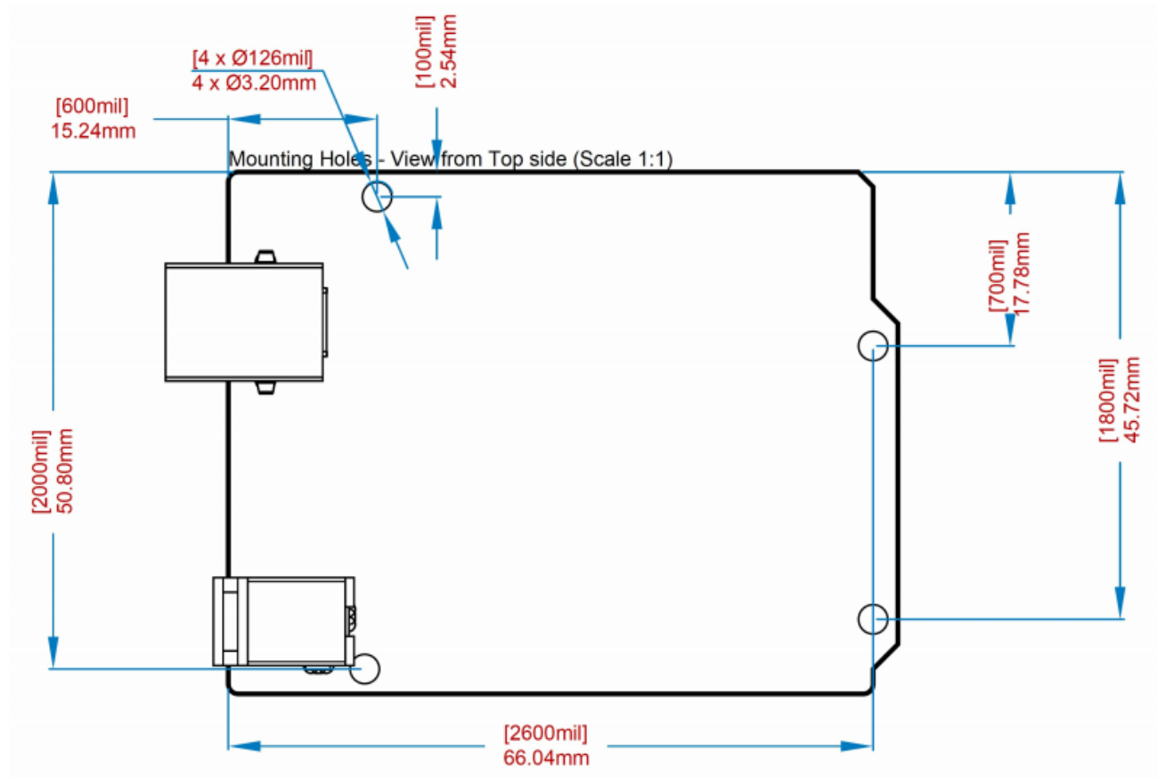
Board outline
