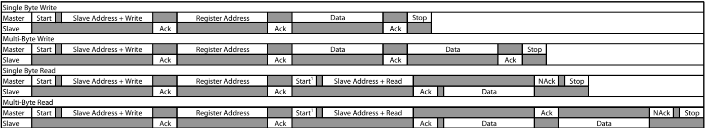
Figure 9. I 2 C Timing Diagram
