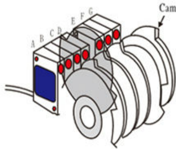
2、Action sequence cam detection
