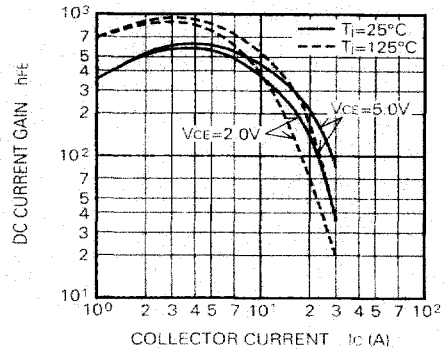
DC CURRENT GAIN VS. COLLECTOR CURRENT (TYPICAL)
