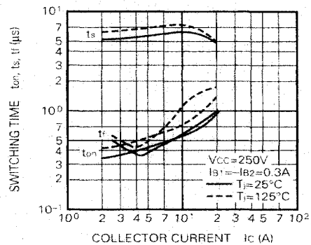
SWITCHING TIME VS. COLLECTOR CURRENT (TYPICAL)
