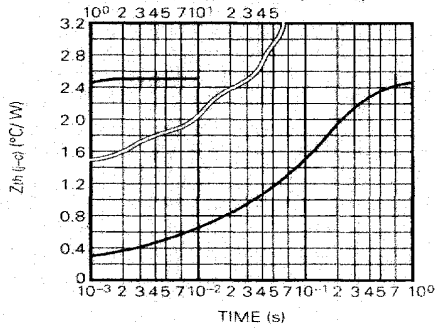
TRANSIENT THERMAL IMPEDANCE CHARACTERISTIC (DIODE)
