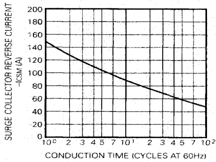
RATED SURGE COLLECTOR REVERSE CURRENT (DIODE FORWARD SURGE CURRENT)
