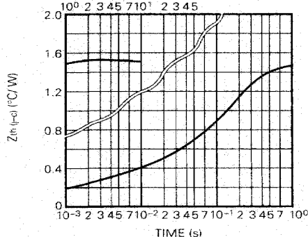
TRANSIENT THERMAL IMPEDANCE CHARACTERISTIC (TRANSISTOR)
