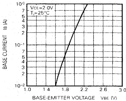
COMMON EMITTER INPUT CHARACTERISTIC (TYPICAL)
