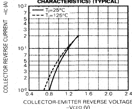
REVERSE COLLECTOR CURRENT VS. COLLECTOR-EMITTER REVERSE VOLTAGE (DIODE FORWARD CHARACTERISTICS) (TYPICAL)
