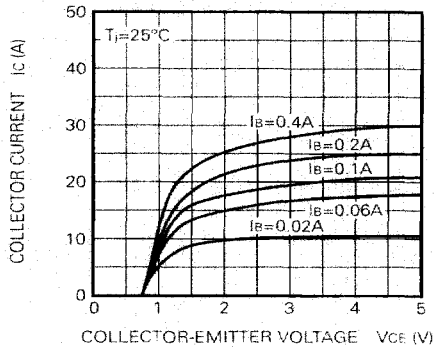
COMMON EMITTER OUTPUT CHARACTERISTICS (TYPICAL)
