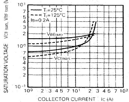
SATURATION VOLTAGE CHARACTERISTICS (TYPICAL)
