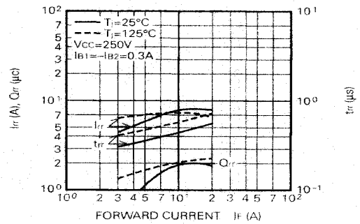
REVERSE RECOVERY CHARACTERISTICS OF FREE-WHEEL DIODE (TYPICAL)
