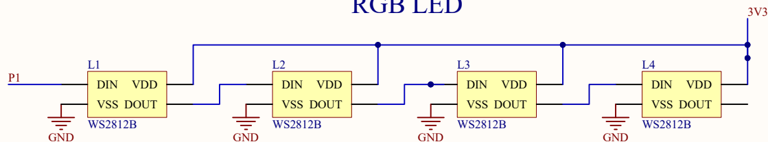
RGB LED
