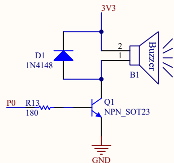
Buzzer
