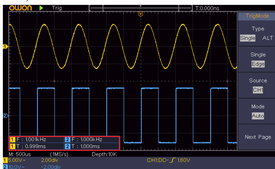
Figure 4-12 Automatic measurement
