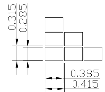
Pixels Details Scale=20/1
