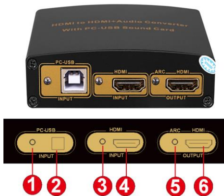
Figure 1.0 Front panel diagram
